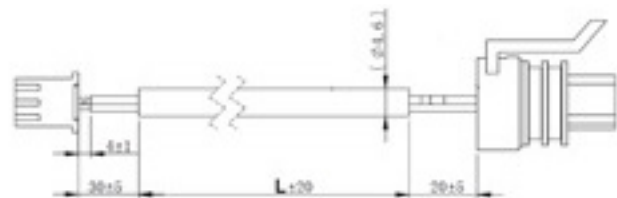
Packard Cables IP 67 + XHP connector with 3 wires
