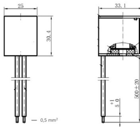
Bistable Coils (SQ-A/D27 Series)
