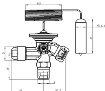
Valve Body - Connection Type: flare/flare/flare
