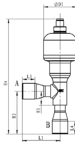
VPF12.5, VPF25, L-Shape version
