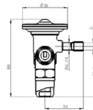
Valve Body - Connection Type: flare/solder/solder
