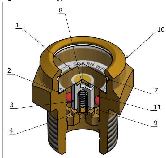
Figure 5: Socket type
