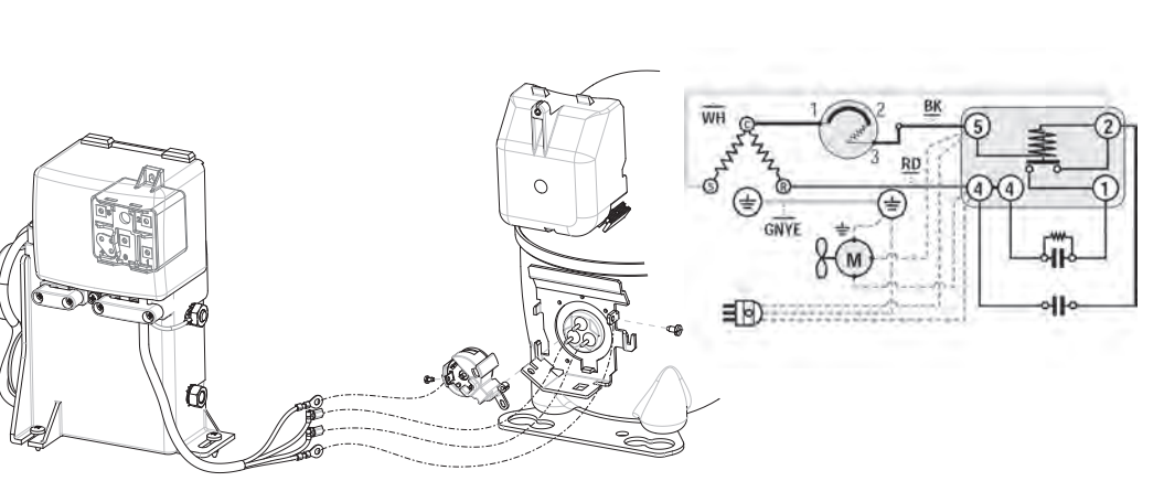
SM06 - NE SERIES CSR Box
