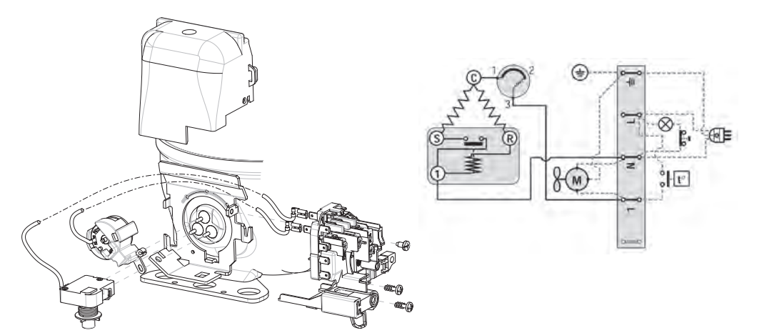
SM03 - EMT/NE SERIES RSIR Terminal Board & Start Device
