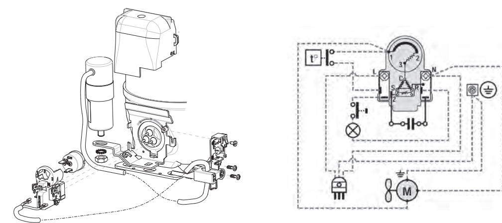
SM02 - EMT/NE SERIES RSCR TSD European Version
