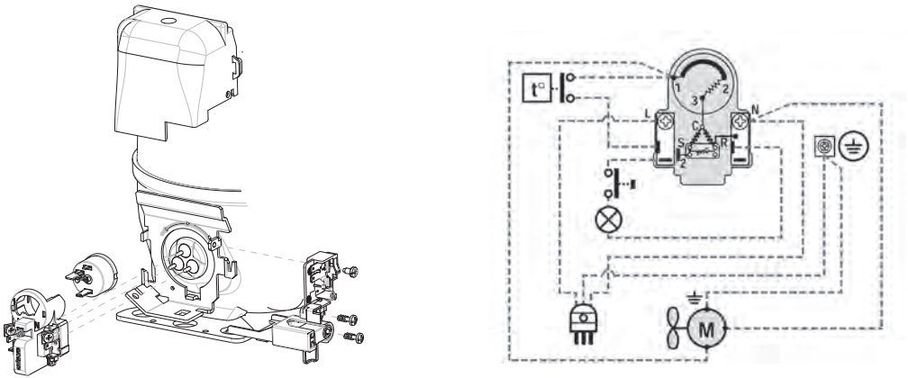
SM01 - EMT/NE SERIES RSCR PTC European Version
