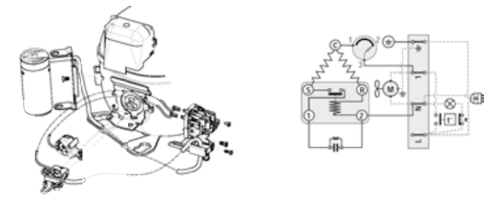
SM19 - UNT SERIE CSIR TERMINAL BOARD
