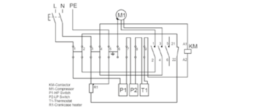
SM28 - SLIDING UNIT CONNECTION
