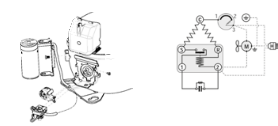
SM20 - UNT SERIE CSIR AMERICAN VERSION
